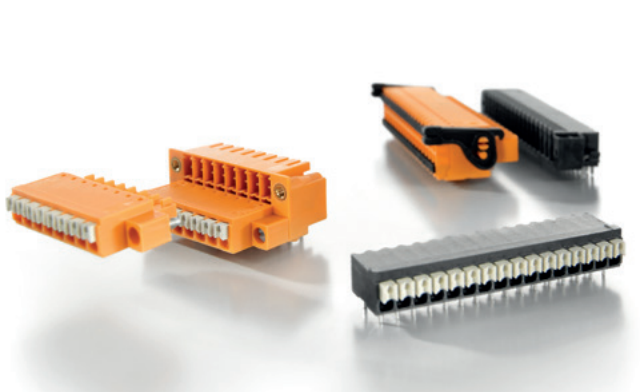
Compact PCB components with a 3.5 mm pitch, in part also with a double-row "PUSH IN" connection
