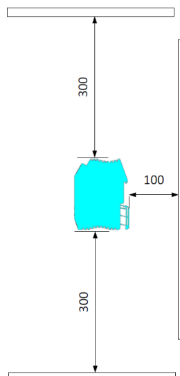
Fig 5: recommended clearance (in mm) to TOP/BOTTOM wall/element and rear wall/element
