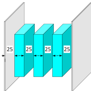
Fig 1: minimum clearance (in mm) between modules and/or other side elements
