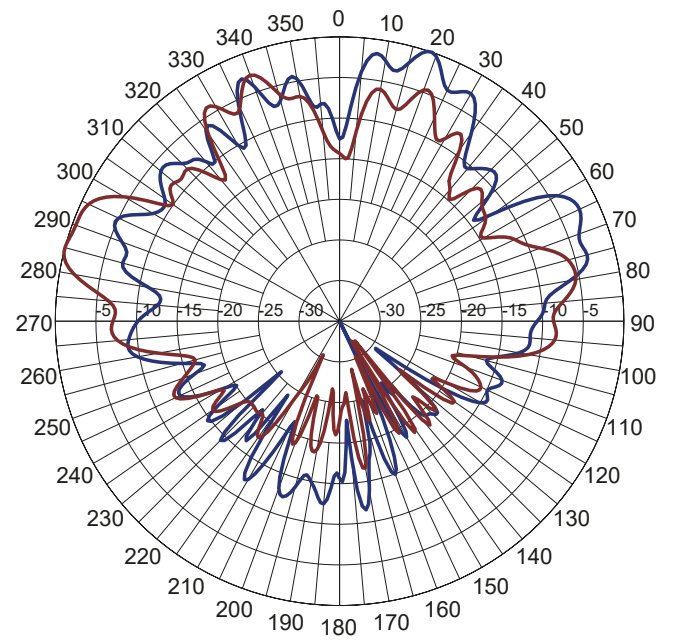
5400 MHz Elevation
