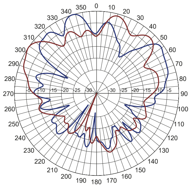
2450 MHz Elevation
