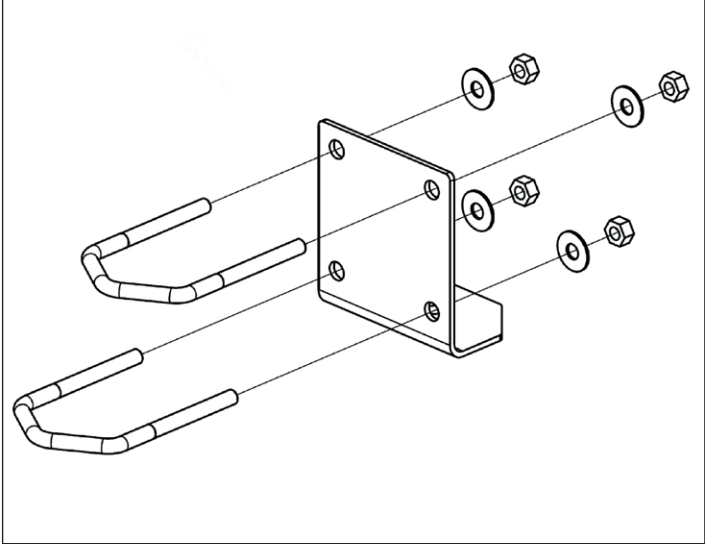
Montage / Mounting
